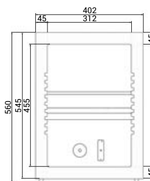
bokorys TM 42
