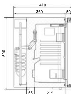
bokorys TM 32
